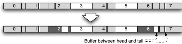
(a) Bands filled with circular logs. Bands 2 and 6 are cleaned, moving their free space buffers to the right within each band, and potentially increasing the size of the buffers by not copying “dead” blocks from tail to head.
