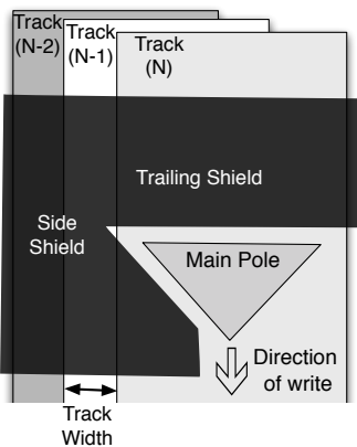
Fig. 1. Corner write head for shingled writes [1].
